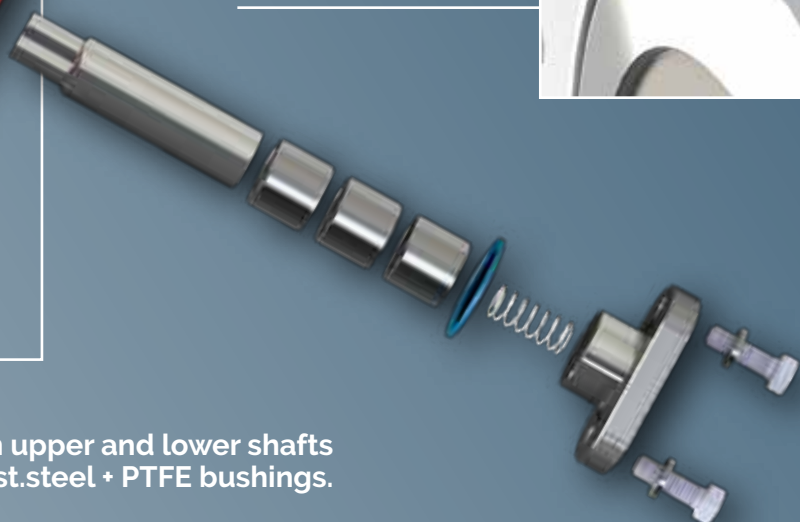
Detail of the Fire Safe design
