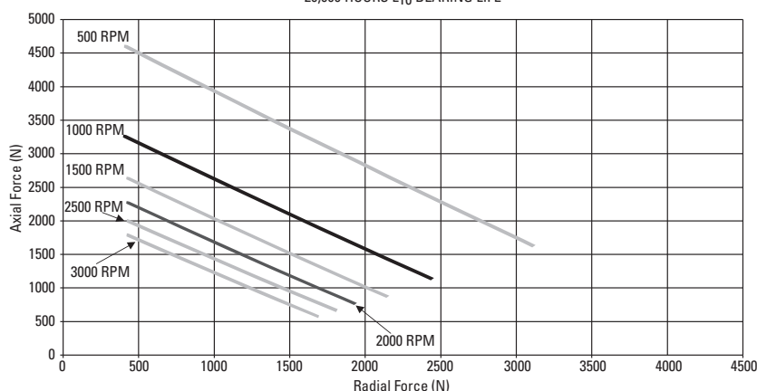
AKM83 & 84 MOTOR WITH REINFORCED BEARING 20,000 HOURS L 10 BEARING LIFE
