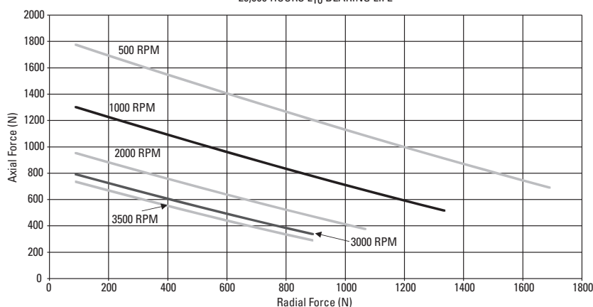
AKM8 MOTORS 20,000 HOURS L 10 BEARING LIFE
