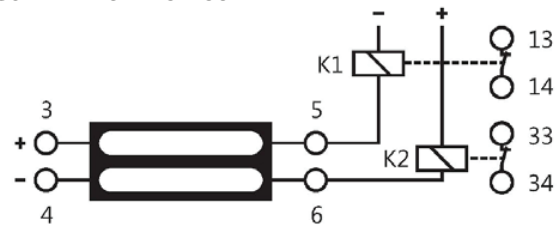
FIGURE 2 INACTIVE SENSOR ELEMENT
