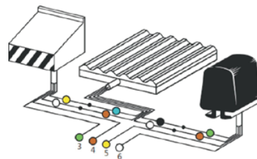
Wiring example for different SSZ products
