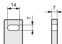
Enlarged view of bracket section
