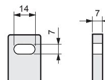
Enlarged view of bracket section
