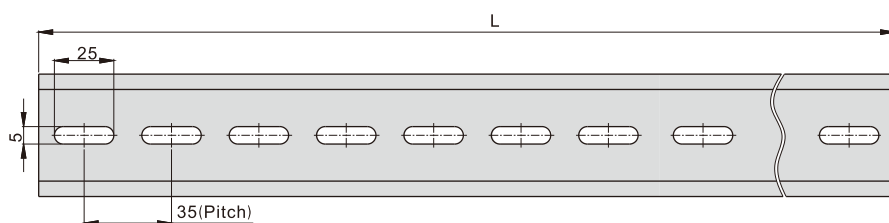
6HV100M11F~24F Guide rail
