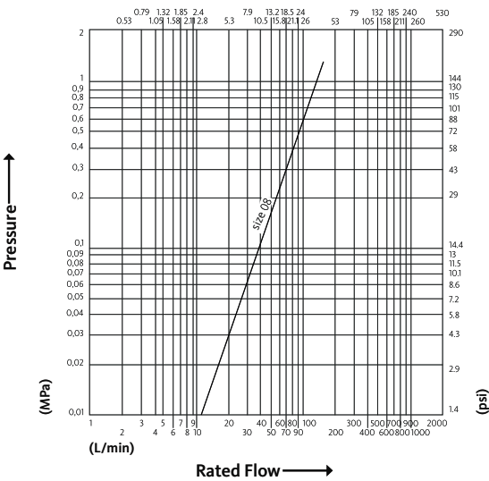
Pressure Drop
