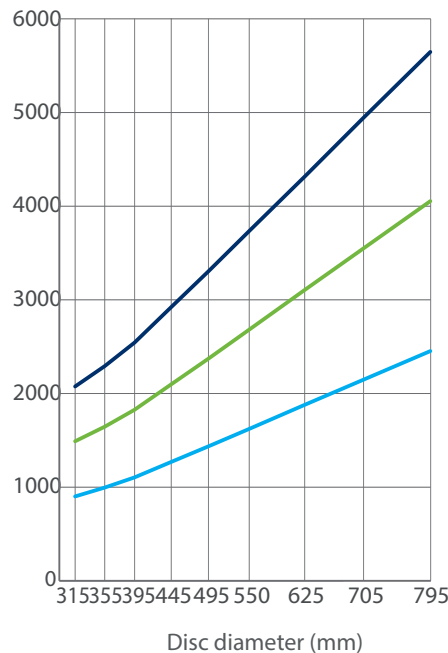
Braking Torque (N.m) (3 types of spring)
