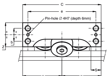
MBL(R) 335-1 (carriage with 1 guide roller on the fixing side)
