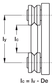
Guide between the rollers
