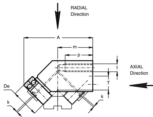
MBL(R) 335-... (carriage with three guide rollers)
