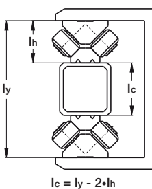
Guides between the rollers
