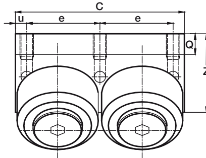
BL 4... four guide rollers block
