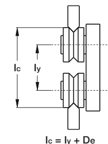
Guides outside the rollers
