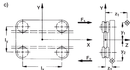
Diagram c) load F applied parallel to axis X
