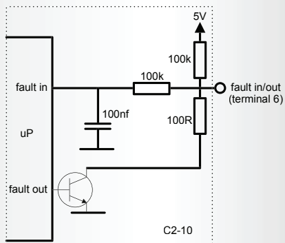
FIG. 2 CIRCUIT DIAGRAM
