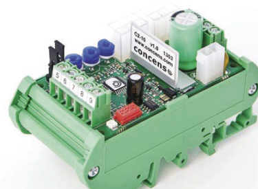
C2-10-DIN (DIN rail version) 90 x 46 x 56 mm (L x W x H)
