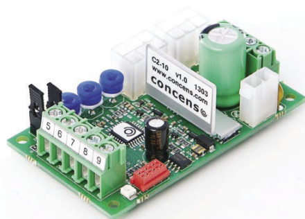
C2-10 (board alone) 73 x 43 x 25 mm (L x W x H)
