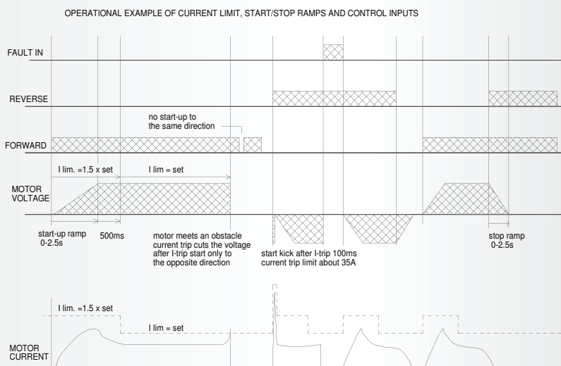
FIG. 4 TIMING DIAGRAM
