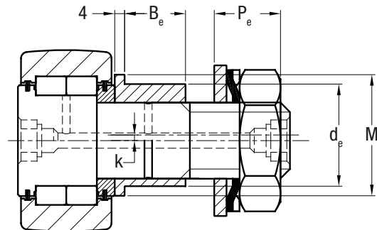
from GCUR62.. to GCUR130..
