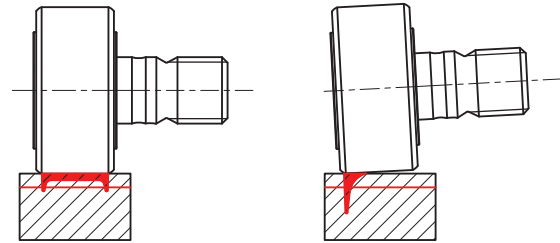
Rollers with cylindrical outer ring
