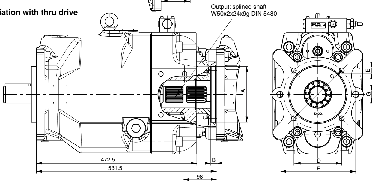
Thru drive adaptors are available with the following dimensions
