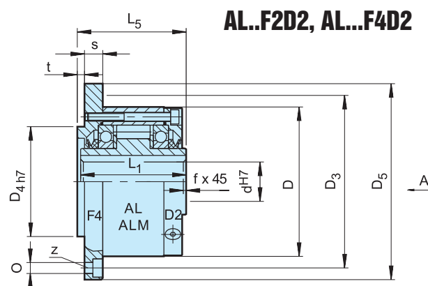
AL..F4D2
