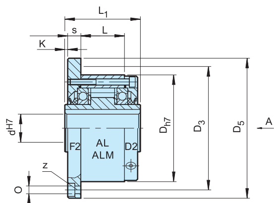
AL..F2D2
