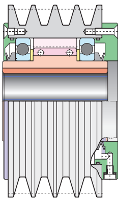
Self-contained freewheel and v-belt pulley assembly
