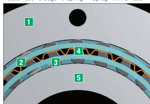
1 Outer race 2 Cage 3 Spring 4 Sprag 5 Inner race
