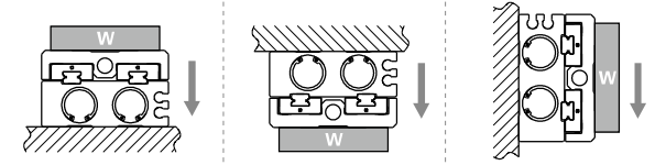
Fig. 1: Applied load
