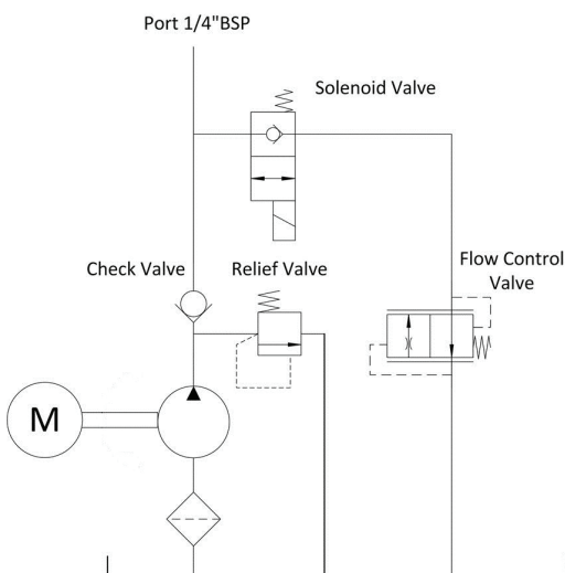
Hydraulic Circuit—Standard
