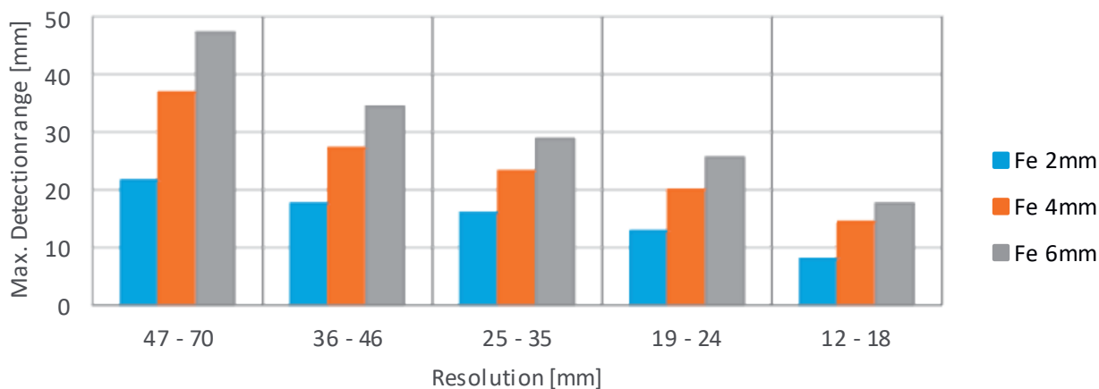
Maximum Detectionrange (Stainless - Threshold typ. 20)
