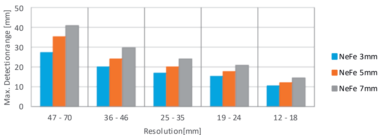
Maximum Detectionrange (Non-Ferrous - Threshold typ. 20)
