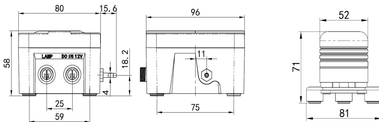
Alarm Box
