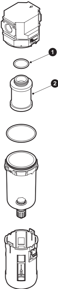
●SFC420 Series
