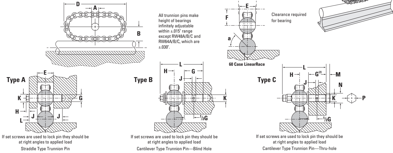
RoundWay Linear Roller Bearing (Type A, B and C) and 60 Case LinearRace (Dimensions in inches)
