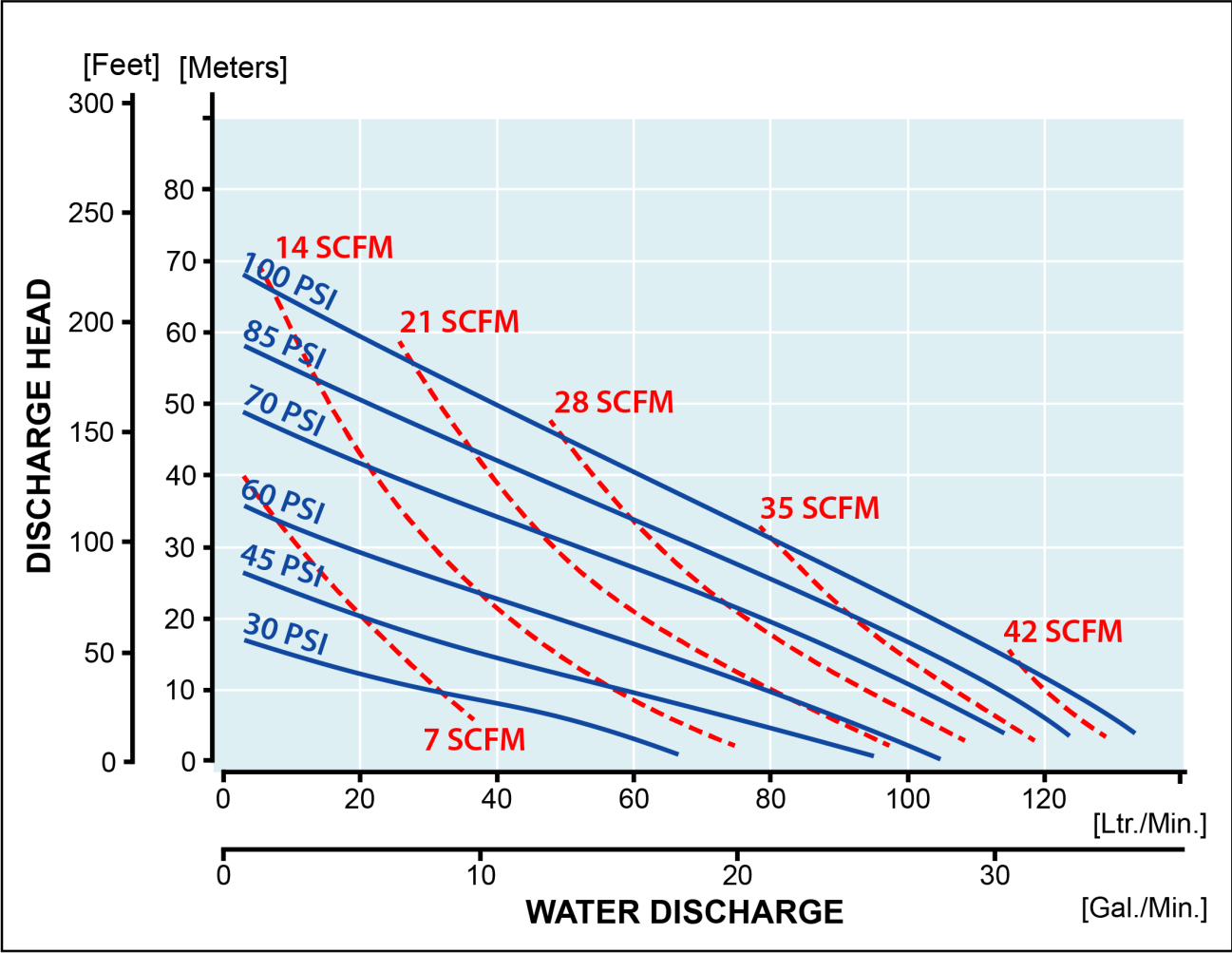
PTFE Diaphragm Performance Curve
