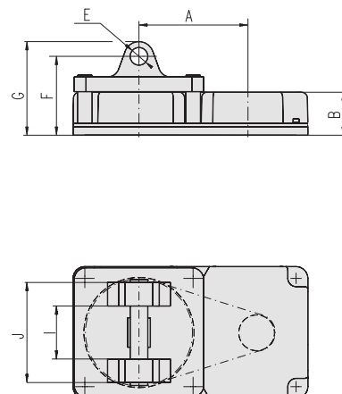
BGM06/81 - CLEVIS OPTION TYPE R
