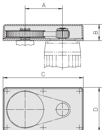
BGM06/09/41/81 - NO CLEVIS OPTION
