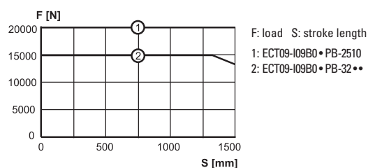
Column Load Limit vs. Stroke
