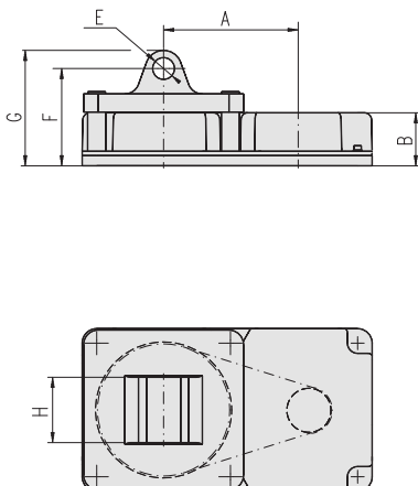
BGM09/41/81 - CLEVIS OPTION TYPE S
