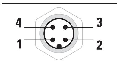
Schematic drawing of M12 plug
