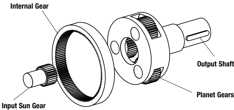
DuraTRUE 90 right angle planetary gearhead
