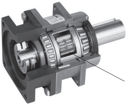
Planetary Gearing
