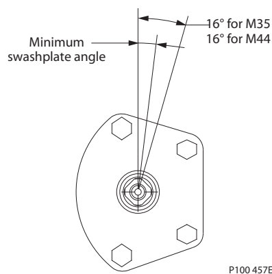
DDC on left side of M35 motor
