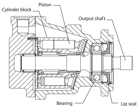
M35/M44 fixed motor (MF)
