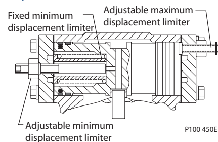
Displacement limiter M46 MV
