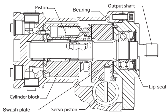
M46 variable motor (MV) (SAE flange)
