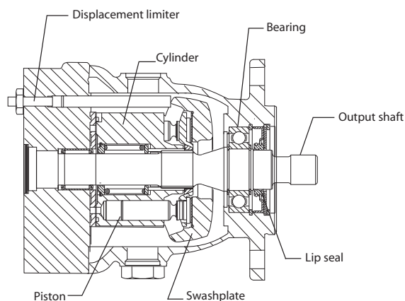
M46 variable motor (MV) (SAE flange)
