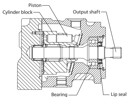
M35/M44 fixed motor (MF)
