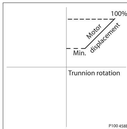
Motor displacement vs swashplate rotation
