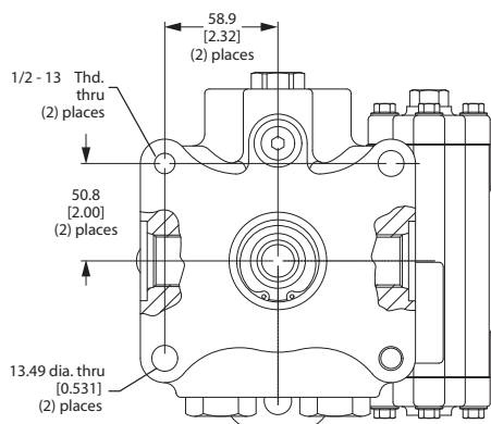
Side ports w/ thru shaft
