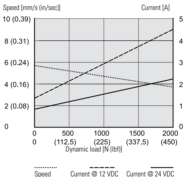
Speed and Current vs. Load
