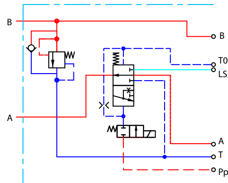
Multi-valve schematic
