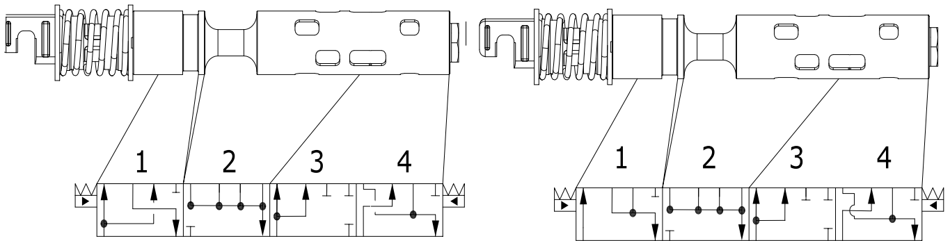
OC-HPCO Spool schematic
