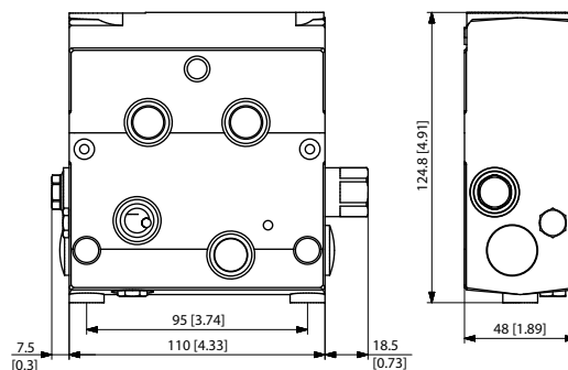
PVSP dimensions
