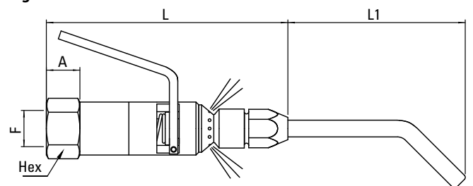
Figure 2 Series 100
