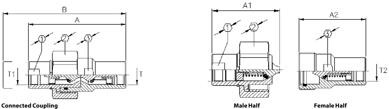
Connected Coupling
