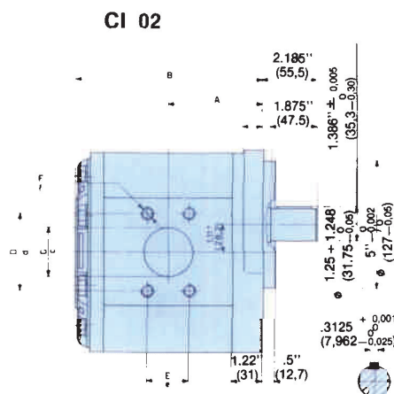
Parallel Shaft
