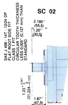
Splined shaft
