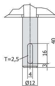
Round shaft with feather key (Option)
