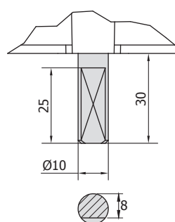
D shaft (Option)
