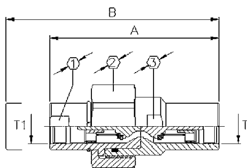
Connected Coupling
