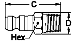
Figure 4 (Tru-Flate)
