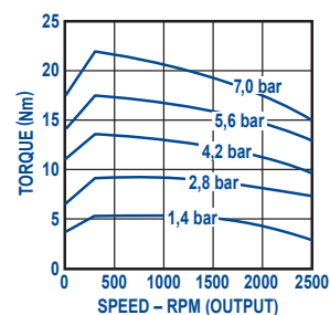
Torque vs. Speed
