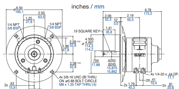
NEMA 56C, U.S. - (NL32-NCC-5, NL32-NCW-6) D71 Flange, Metric - (NL32-NCC-7, NL32-NCW-8)
