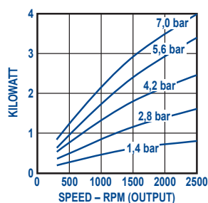
Output Power vs. Speed
