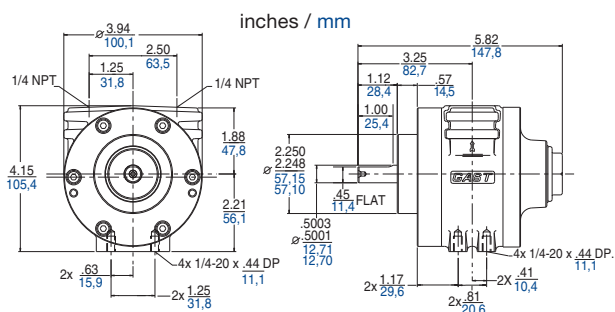
Hub mounting (NL32-NCC-1, NL32-NCW-2)
