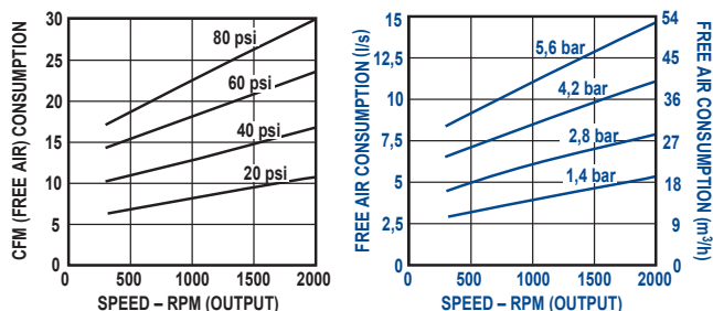
Air Consumption vs. Speed
