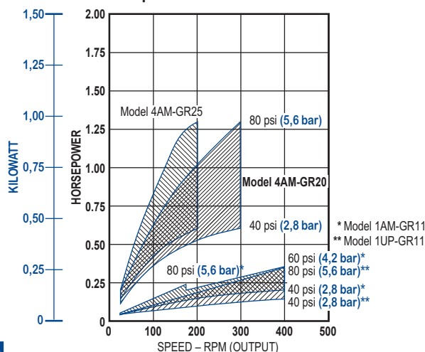
Spur Gearmotor
