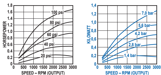
Output Power vs. Speed
