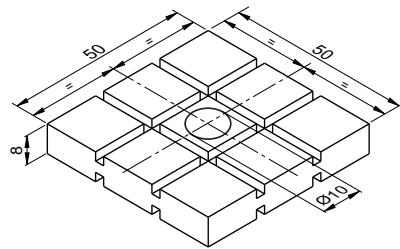
Antivibrationsunterlage aus Nitrilkautschuk Nitrile rubber isolation pads
