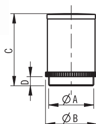
Filtering net and cover in stainless steel (AISI 304) Threaded connection in Nylon (PA)
