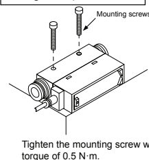
Bracket mounting (use of dedicated bracket)
