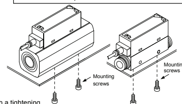
Vertical mounting (use of female thread on bottom surface)
