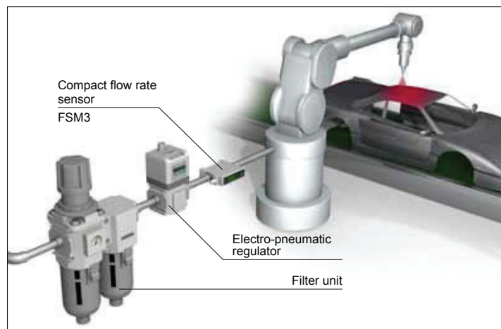
Electro pneumatic regulator
