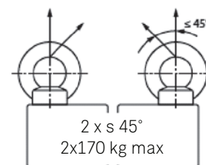
load capacity /using bolt
