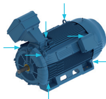
Figure 3 - Eye-bolt fixing points for motors with feet.
