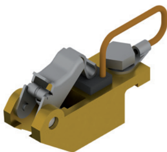
Figure 12 - Shaft grounding brush for bearing.
