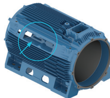
Figure 19 - Air ducts of the frame for air flow.
