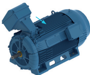
Figure 33 - Airflow channels in the motor frame.
