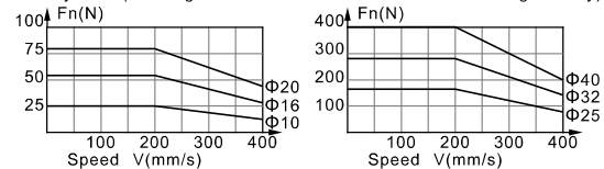
Force-Velocity chart (Pushing force in horizontal movement and moving velocity)
