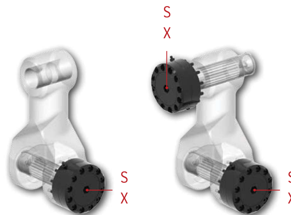
BRAKE STRUCTURE FOR R-LINKS
