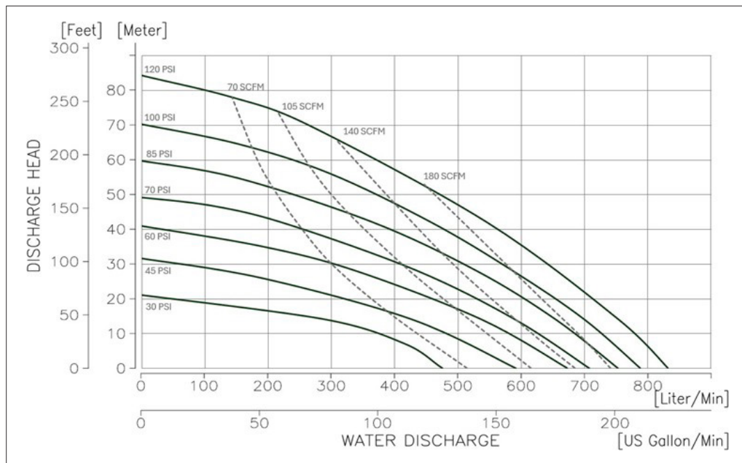
NDP-500 - Rubber Performance Curve
