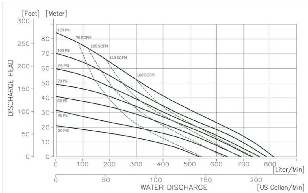
NDP-500 - Ultimate Performance Curve
