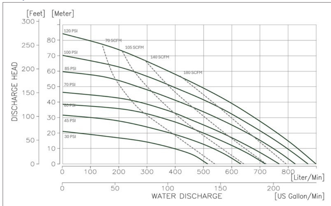
NDP-500 - Thermoplastic Performance Curve
