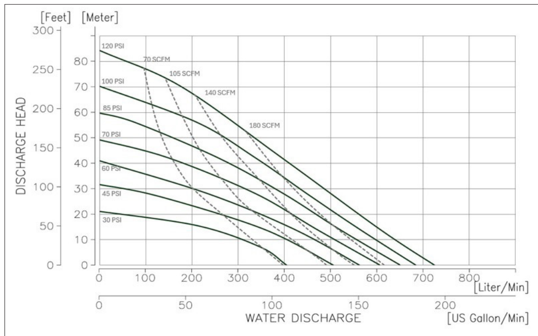
NDP-500 - PTFE Performance Curve
