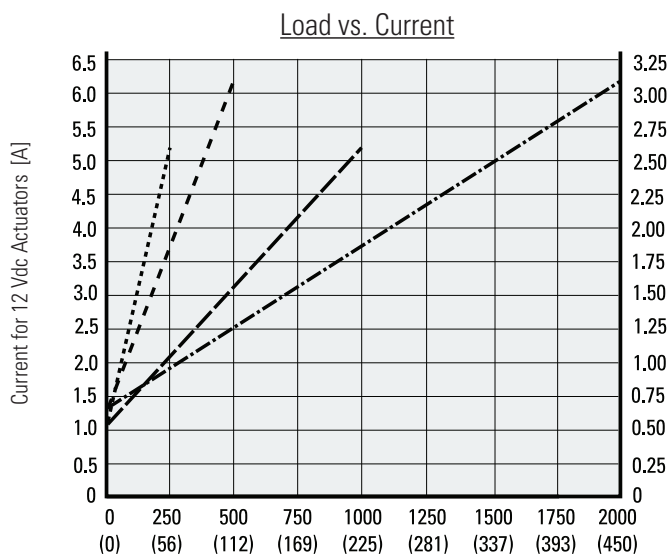
Dynamic Load Capacity
