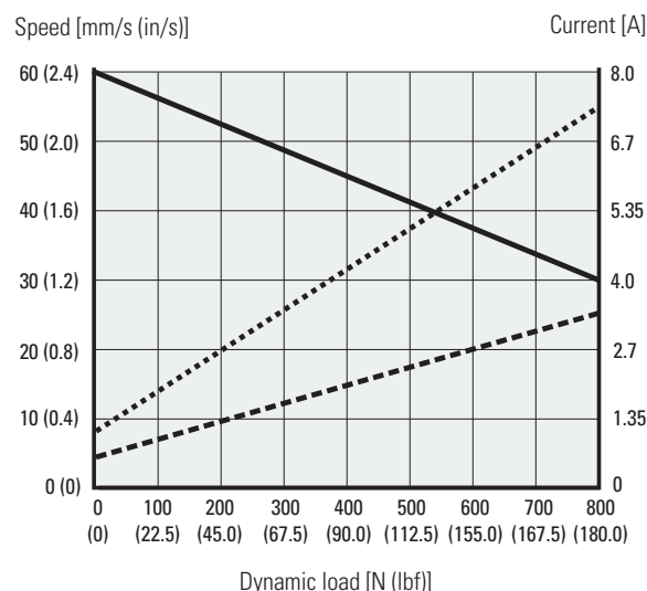
Ball Screw Models (MXxxB)
