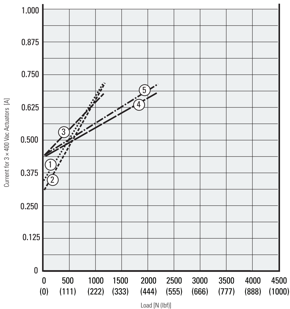
Load vs. Current for 3 × 400 Vac actuators
