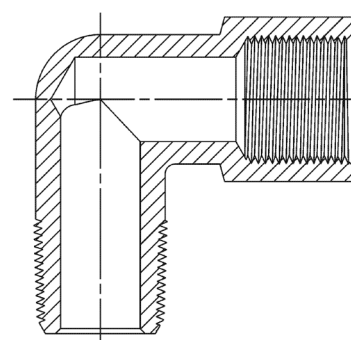
Pipe fittings
