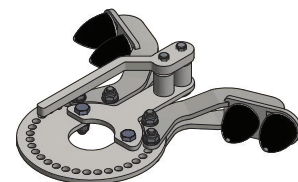
5. Rotation limiter
