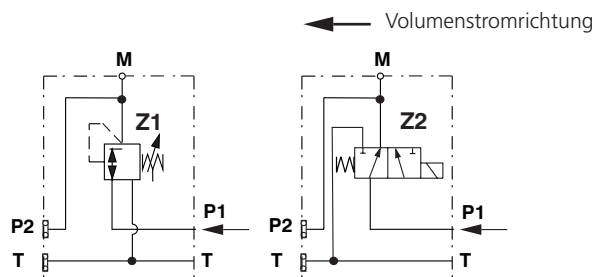
Block HB03-RPEK-MP1
