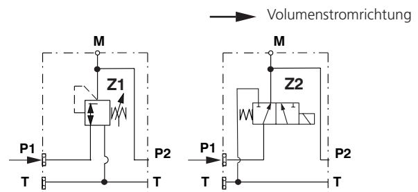
Block HB03-RPEK-MP2
