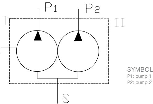
EXAMPLE OF A CONNECTION DIAGRAM The illustration on the left shows a connection diagram with one high pressure and one low pressure pump each. P1: low pressure pump with high capacity P2: high pressure pump with low capacity
