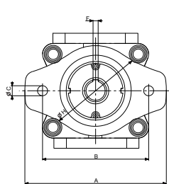
AB PUMP COMBINATION
