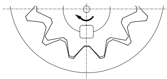
NEW: TRUNINGER TEETH SHAPE OF QX PUMPS
