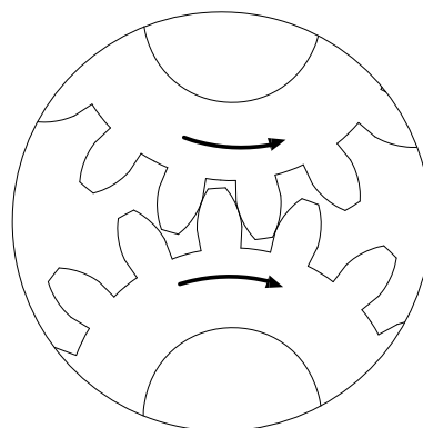
FORMER: INVOLUTE GEAR SHAPE
