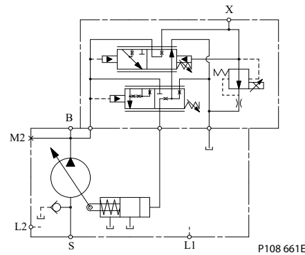
Schematic
