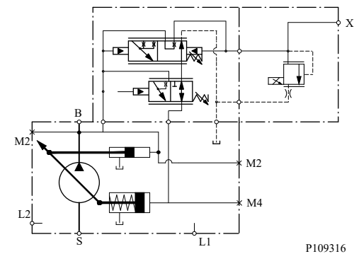
Schematic
