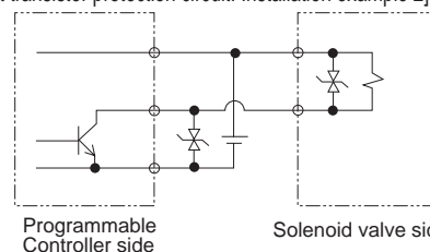
[Output transistor protection circuit: Installation example 2]
