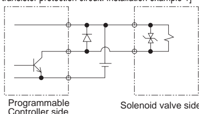
[Output transistor protection circuit: Installation example 1]
