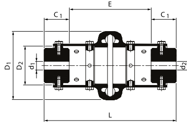
RLU BSB Standart Tip
