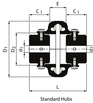
RLU BWB Standart Tip
