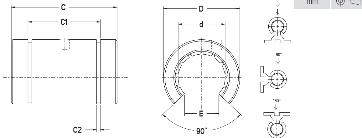
Dimensions [mm]
