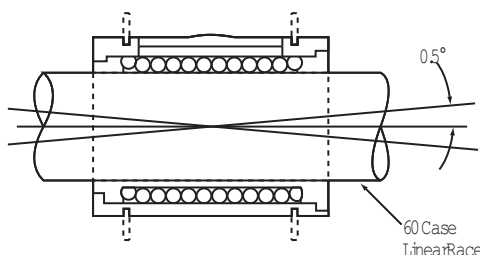
Figure 3 Super Ball Bushing Bearing Self-Alignment Feature
