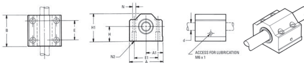
Super Smart Pillow Blocks (Closed Type) (Dimensions in mm)
