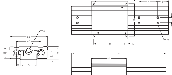
Dual Shaft Rail Linear Guide with Integrated Full Length Carriage
