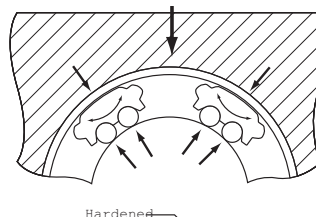
Figure 5 Super Smart Ball Bushing Bearing Self-Alignment Feature
