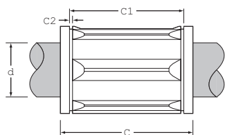
Precision Steel Ball Bushing Bearings (Closed Type) and 60 Case® LinearRace® (Dimensions in inches)
