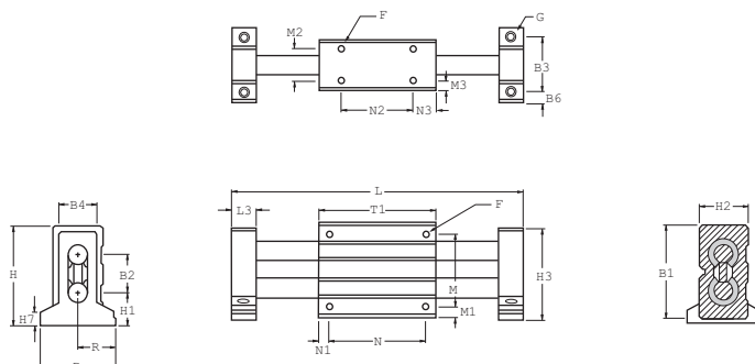
Twin Shaft Web Linear Guide with Universal Carriage (Vertical Configuration)
