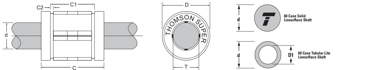
Super Ball Bushing Bearings (Closed Type) and 60 Case® LinearRace® (Dimensions in inches)
