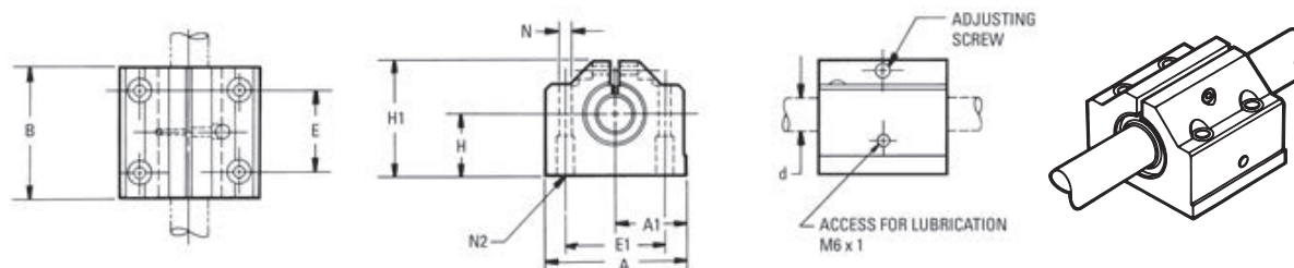
Super Smart Pillow Blocks (Closed Adjustable Type) (Dimensions in mm)
