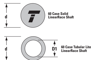
Super Smart Ball Bushing Bearings (Closed Type) and 60 Case® LinearRace® Shafting (Dimensions in inches)
