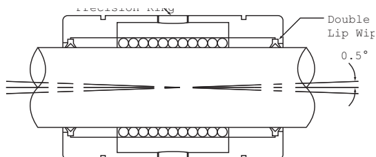
Figure 4 Super Smart Ball Bushing Bearing Self-Alignment Feature
