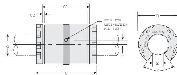
Super Smart Ball Bushing Bearings (Open Type) (Dimensions in mm)
