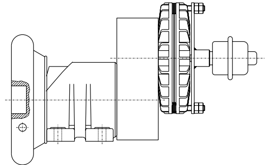
Chuck with ESB brake and intermediate gearbox Info 10.02
