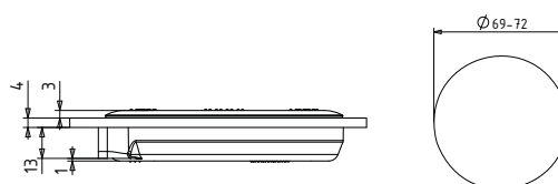
Bohrbild Hole pattern
