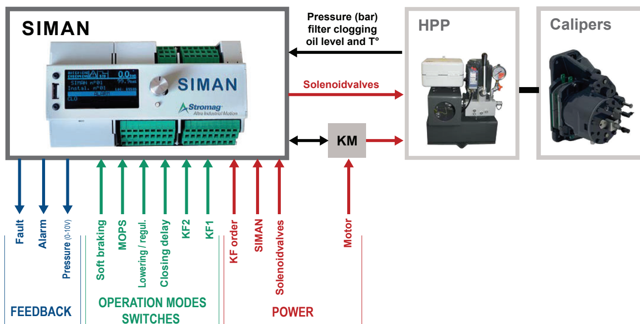
Diagram of the SIMAN inputs and outputs
