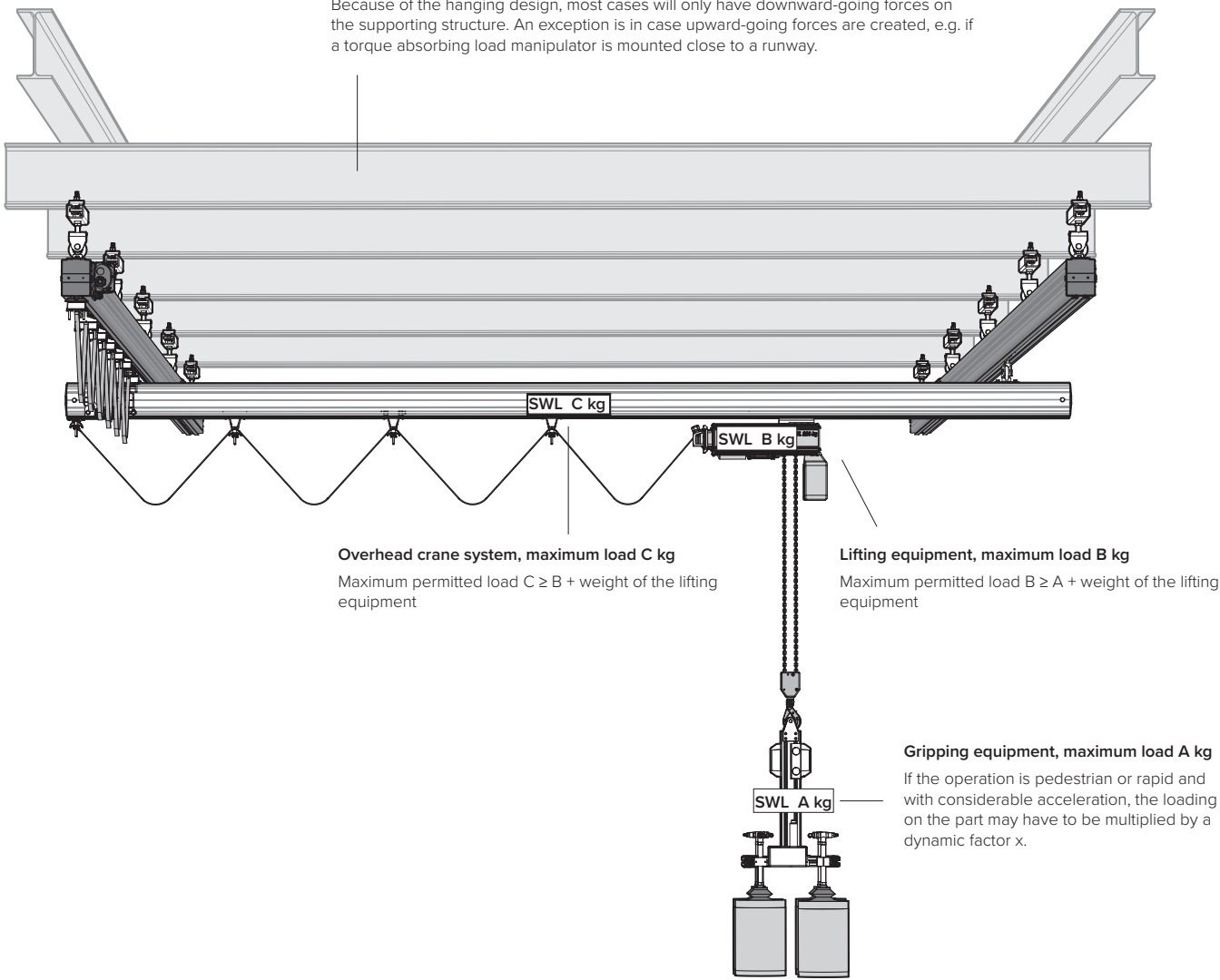
Example of marking for maximum permitted load for each level respectively in a simple ceiling-mounted overhead crane system.
