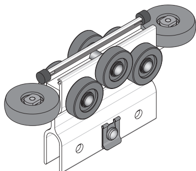
(E) Trolley with nose wheel
