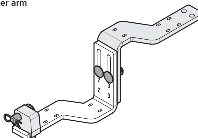
Follower arm
